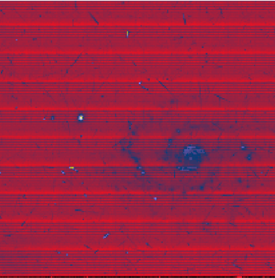
Galaxy M51
